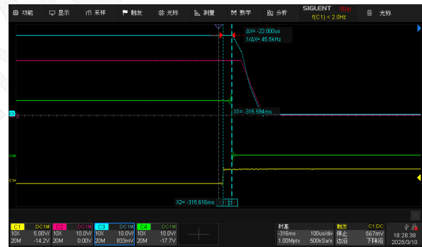
OVLO protection
