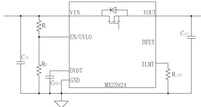
Typical Application
