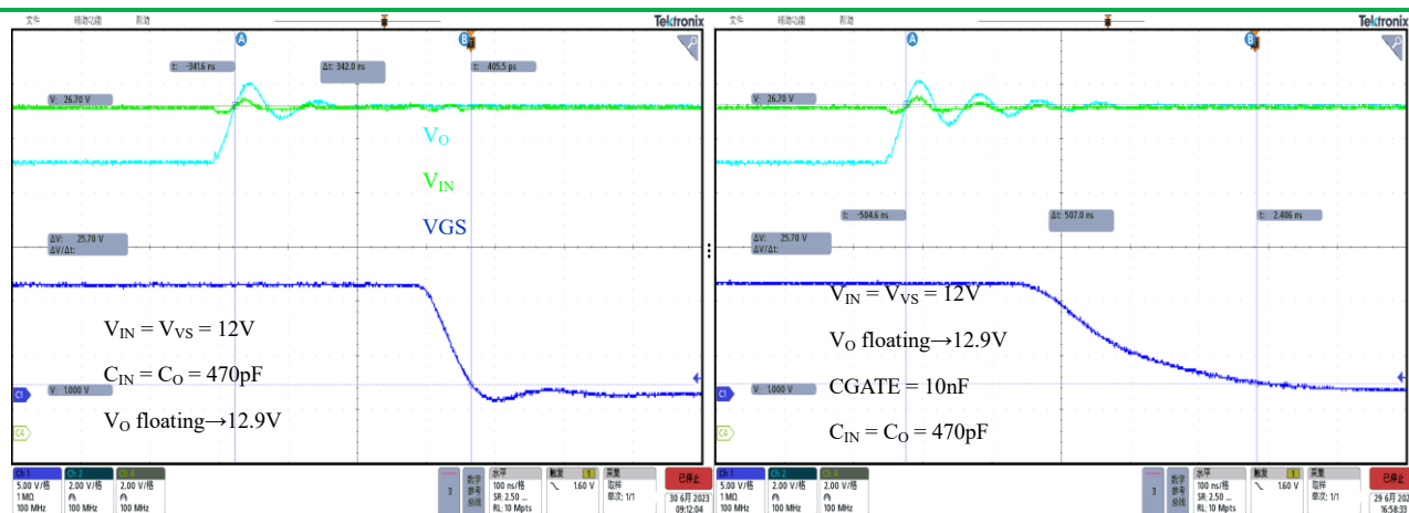
Reverse GATE discharge time
