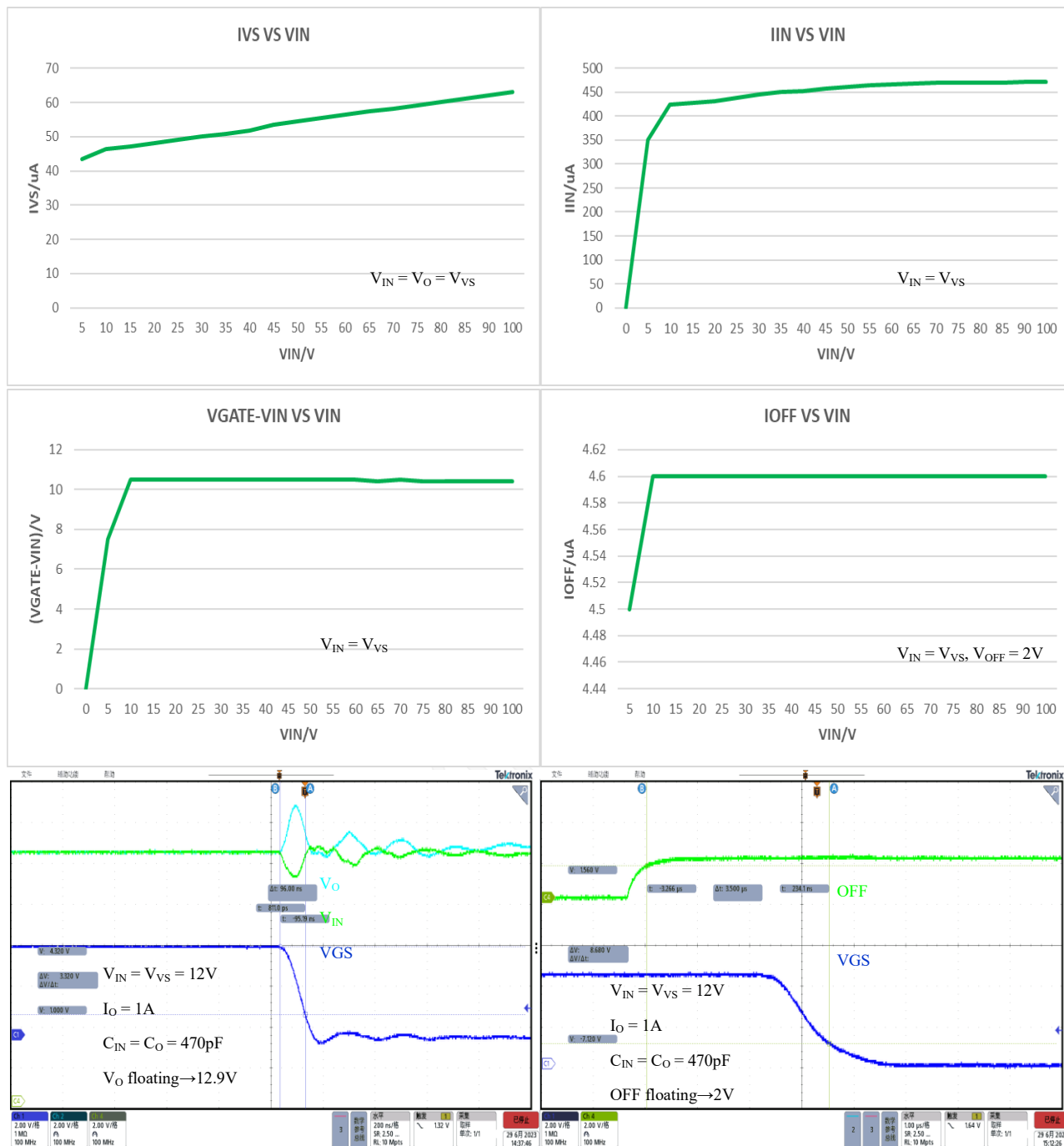
Reverse C_{GATE} discharge time
