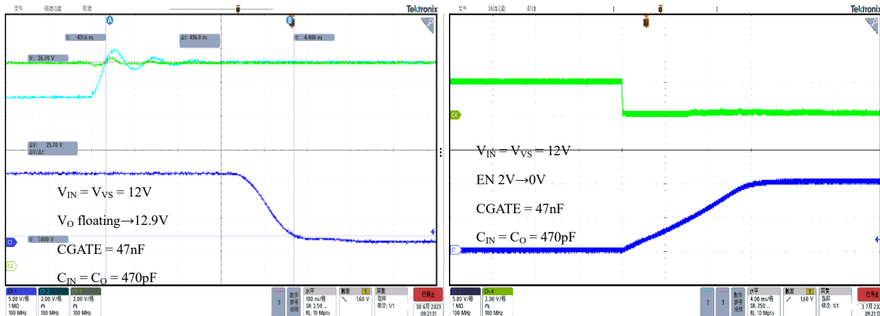
Reverse GATE discharge time, C_{GATE} = 47\text{nF}
