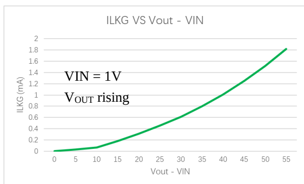
Leakage current with Reverse Polarity
