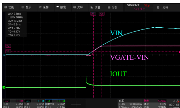
VCAP-VIN During Startup at 3A Load
