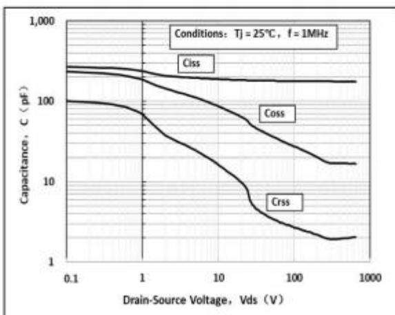
Fig 17: Capacitance Characteristics
