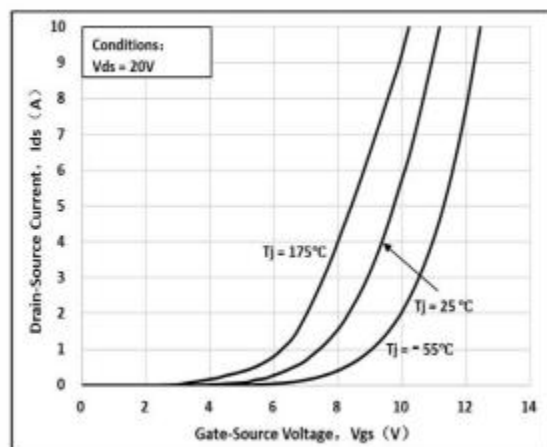
Fig 5: Transfer Characteristic
