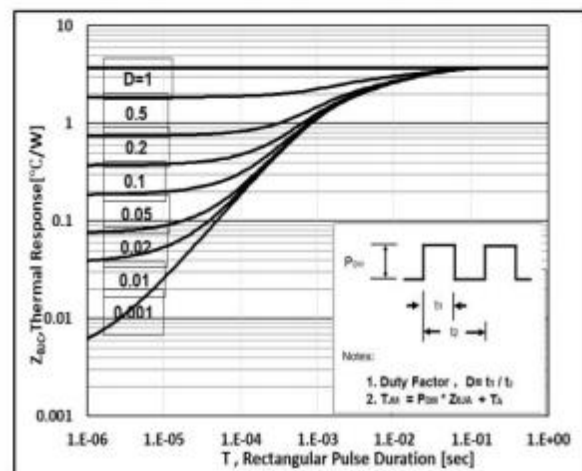
Fig 18: Transient Thermal Impedance
