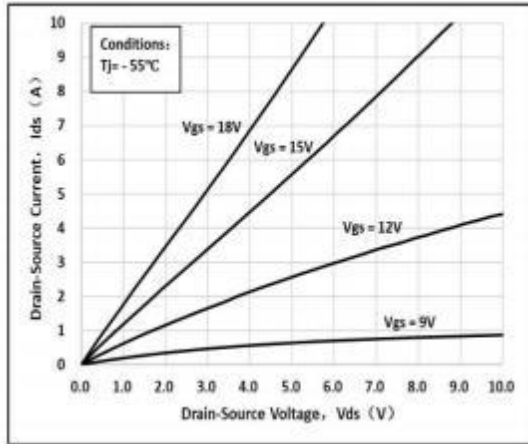
Fig 1. Output Characteristic ( T_J = -55^\circ\text{C} )
