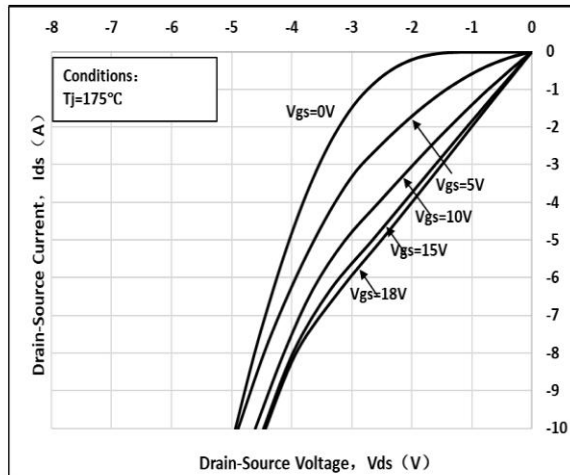
Fig 13: 3rd Quadrant Characteristic( T_J=175^{\circ}\text{C} )
