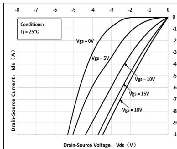
Fig 12: 3rd Quadrant Characteristic ( T_J = 25^\circ\text{C} )
