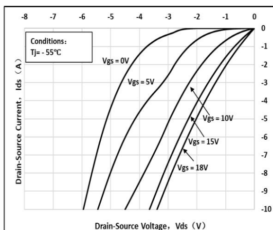
Fig 11: 3rd Quadrant Characteristic ( T_J = -55^\circ\text{C} )
