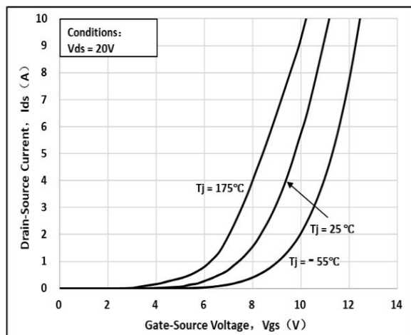
Fig 5: Transfer Characteristic
