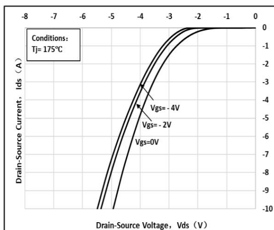
Fig 9: Body-diode Characteristic ( T_J = 175^\circ\text{C} )
