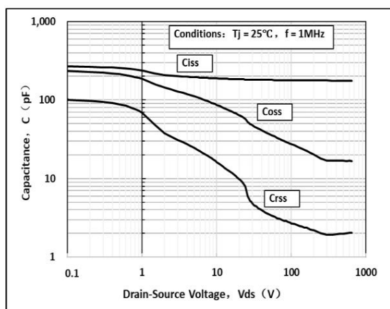
Fig 17: Capacitance Characteristics
