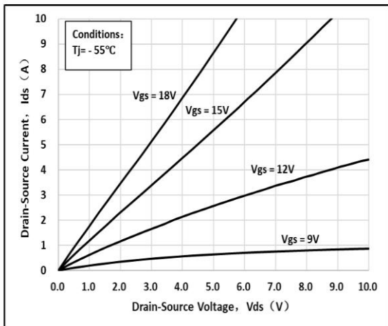
Fig 1. Output Characteristic ( T_J = -55^\circ\text{C} )
