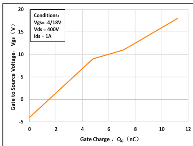
Fig 14: Gate Charge Characteristics
