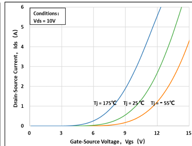
Fig 6: Transfer Characteristic
