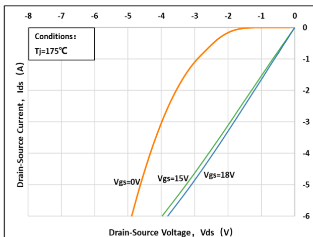
Fig 13: 3rd Quadrant Characteristic( T_J=175^{\circ}\text{C} )
