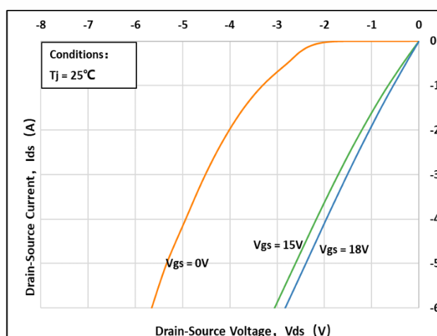
Fig 12: 3rd Quadrant Characteristic ( T_J = 25^\circ\text{C} )
