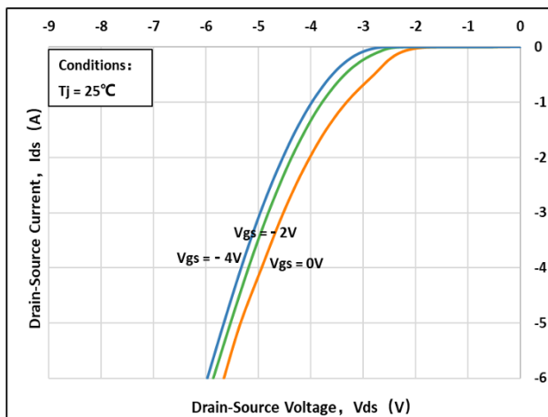
Fig 8: Body-diode Characteristic ( T_J = 25^\circ\text{C} )
