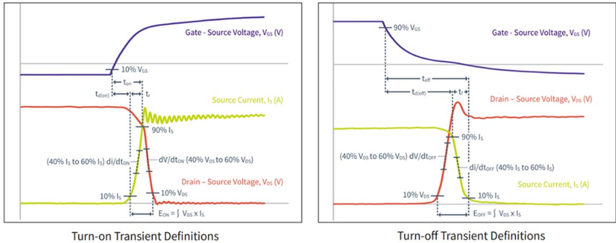
Figure A. Definition of switching times
