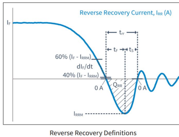
Figure C. Definition of body diodeswitching characteristics
