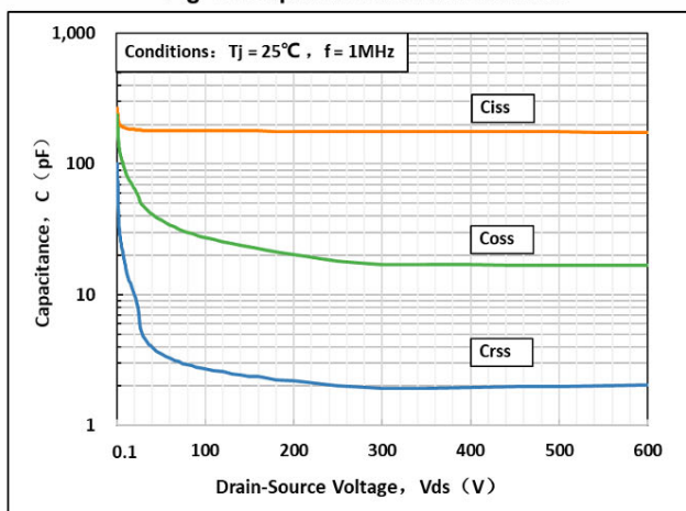
Fig 17: Capacitance Characteristics
