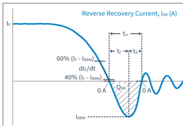
Reverse Recovery Definitions
