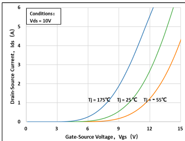
Fig 6: Transfer Characteristic
