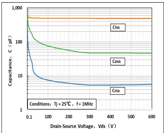
Fig 17: Capacitance Characteristics
