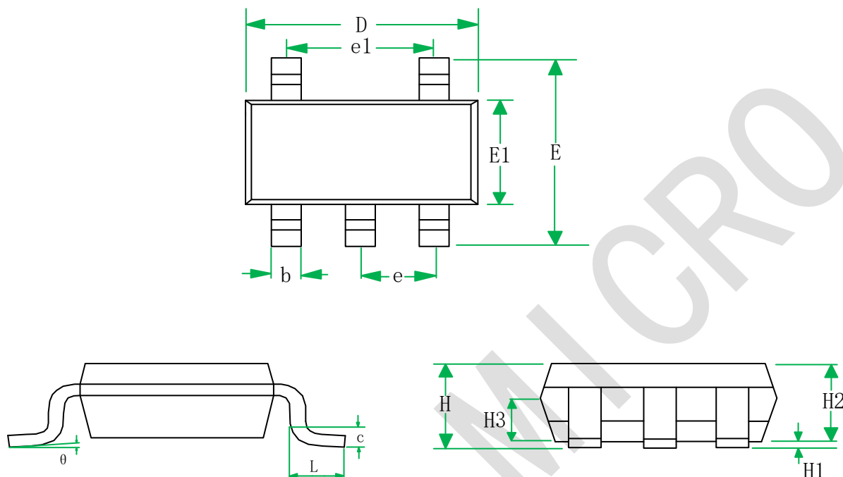
SOT23-5 for MX6288T
