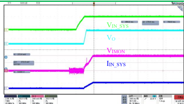
I_{MON} Response During a Load Step
