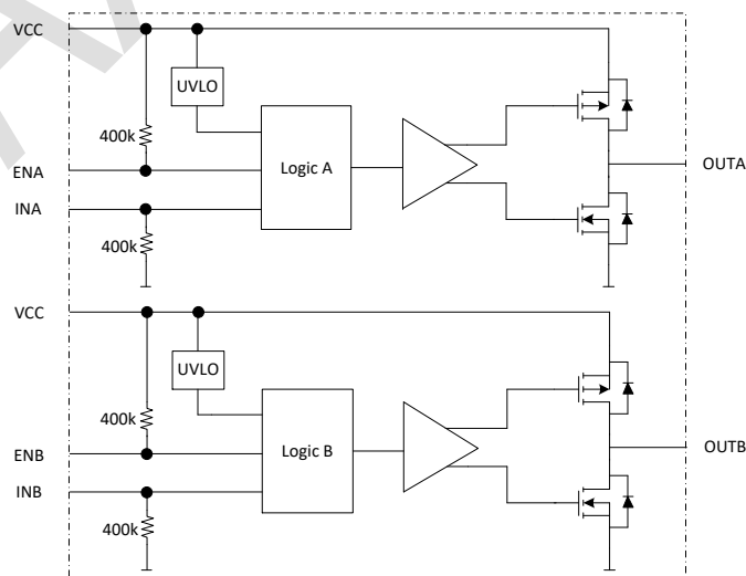
Figure5 block diagram
