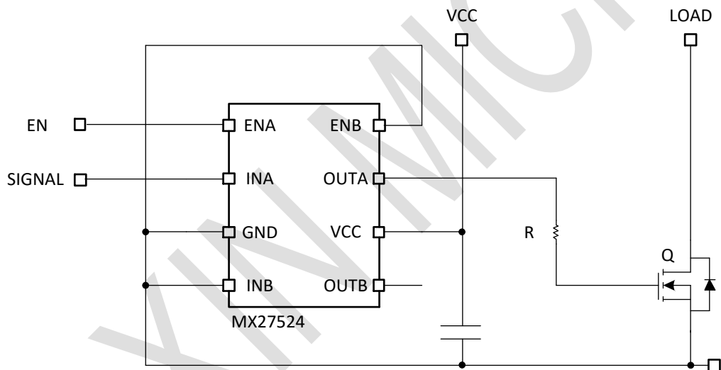
Figure2 MX27524 application for one channel
