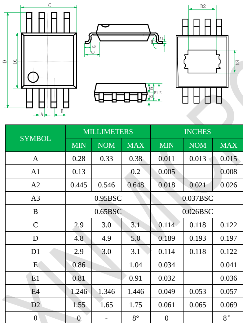
eMSOP8 for MX27524ES
