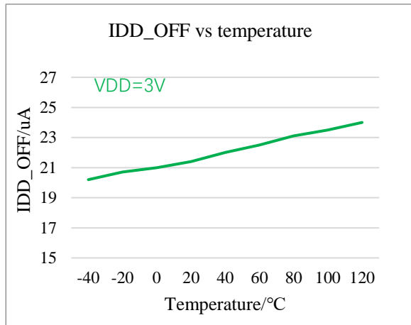
VDD OFF current vs temperature
