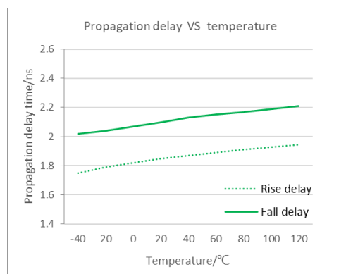
Propagation delay time
