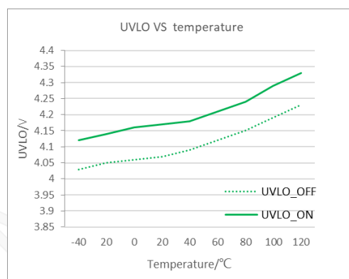
Under voltage
