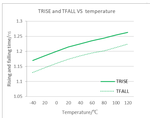
Rising and falling time with 100pF load
