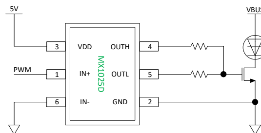
Typical Application
