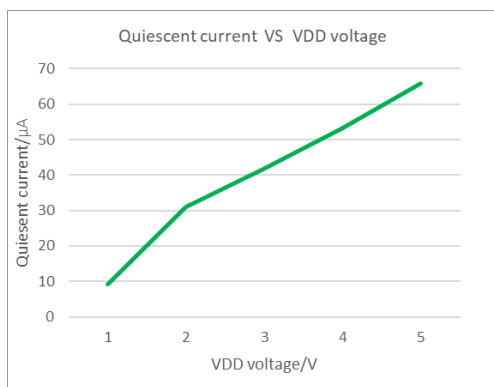
Quiescent current
