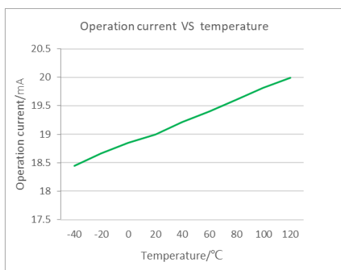
Operation current with 100pF load
