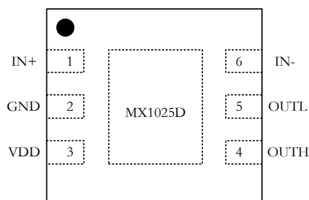
Pin information
