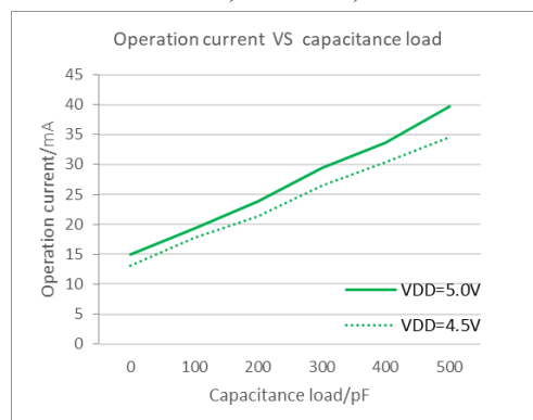
Operation current with different capacitance load
