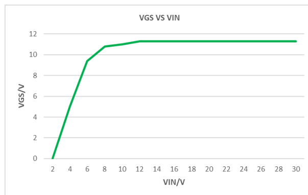
Vgate – Vsource vs Input voltage
