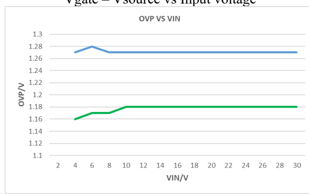
OVP vs Input voltage
