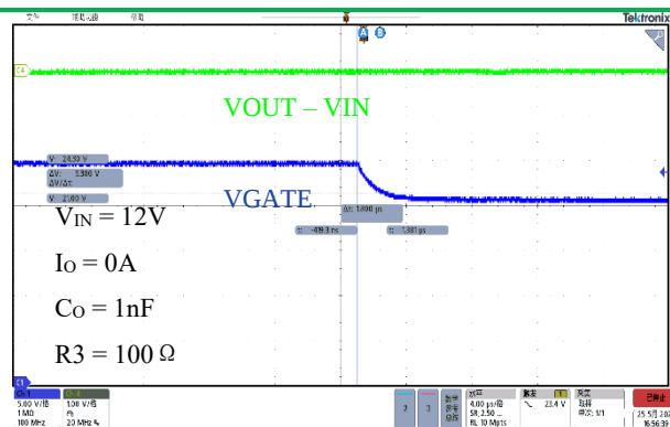
Reverse prtction
