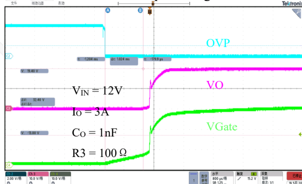
OVP protection release
