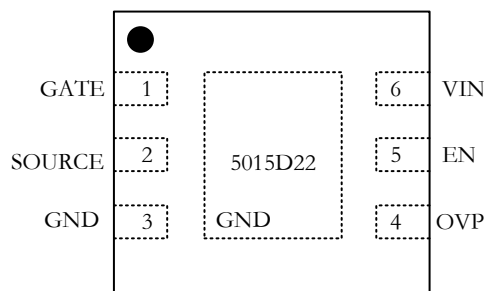
Pin information
