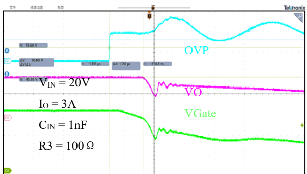
OVP protection
