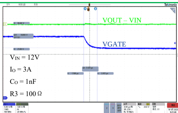
Reverse prtction
