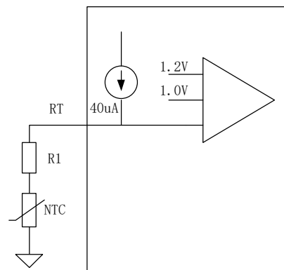
Figure6 external over temperature protection application
