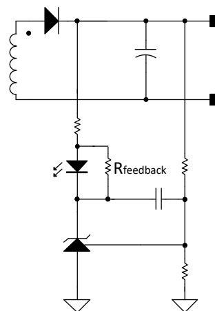
Figure7 Feedback resistor
