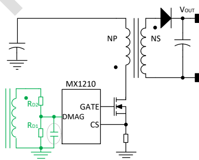
Fig4 DMAG pin application
