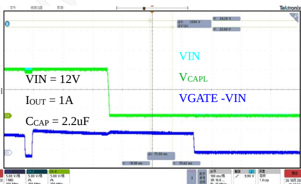
Shutdown Relative to VIN
