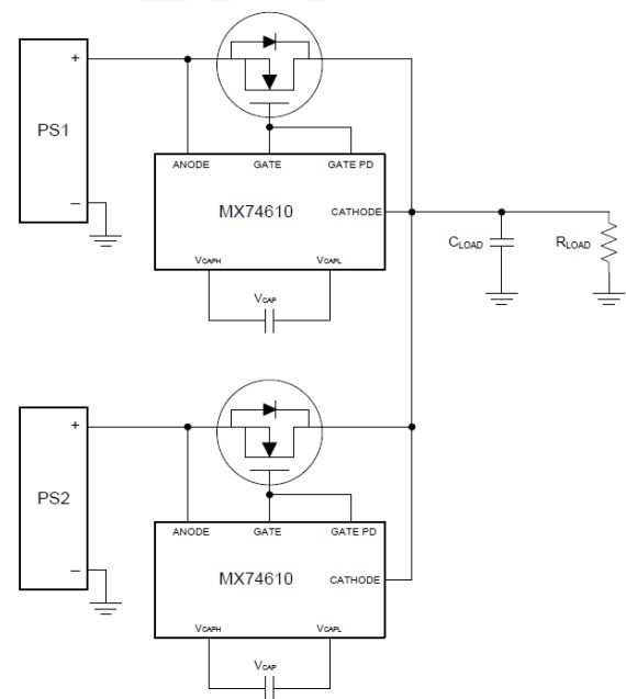
Typical OR-ing Application
