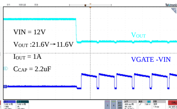
Response to exit reverse Polarity
