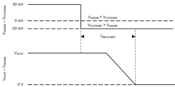
Gate Shut Down Timing in the Event of Reverse Polarity
