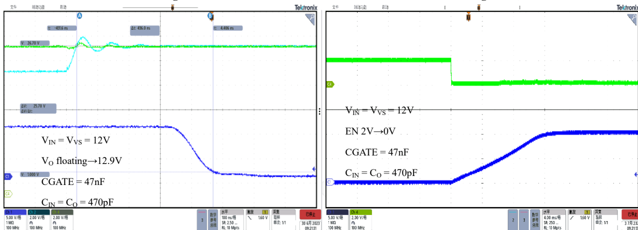
Reverse GATE discharge time, C_{GATE} = 47nF
