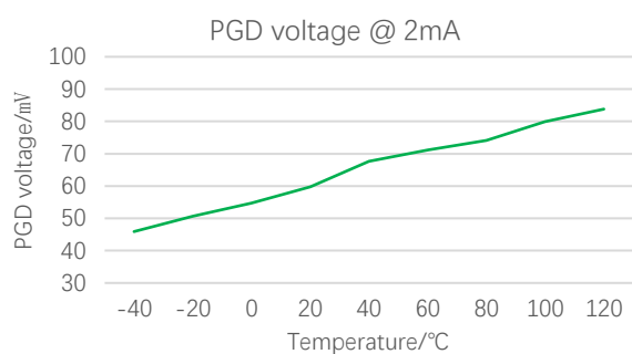
The PGD voltage vs temperature
