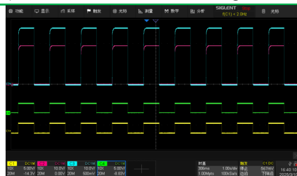
Continues repeated switch on an off with 10A load
