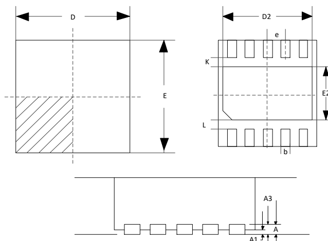
DFN3*3-10L for JMW960DL
