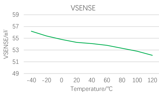
Current limit sense voltage vs temperature
