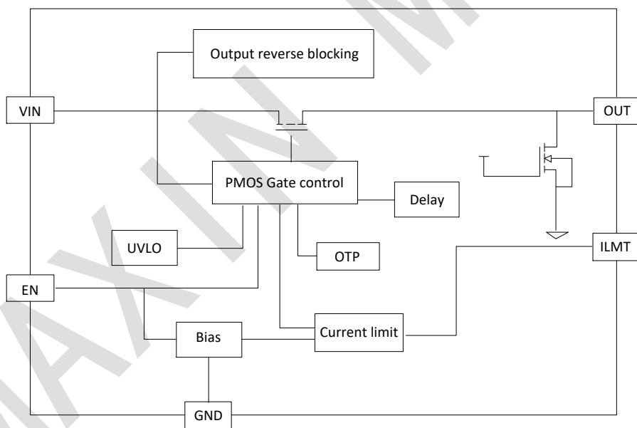
Figure6 block diagram
